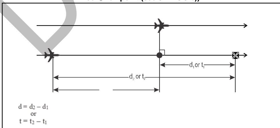
Figure 5-35. Calculation of longitudinal distance/time between aircraft — parallel tracks (see 5.4.2.9.5 c))
