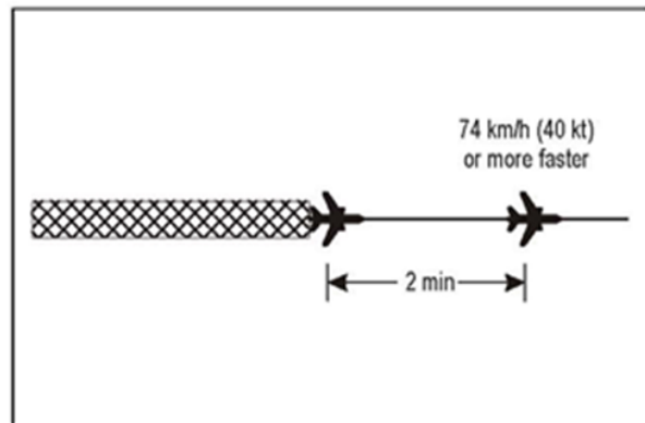
Figure 5-38. Two-minute separation between aircraft following same track (see 5.6.2)
