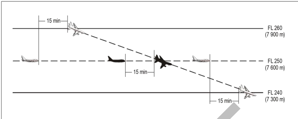
Figure 5-19B. Fifteen-minute separation between aircraft descending and on crossing tracks
