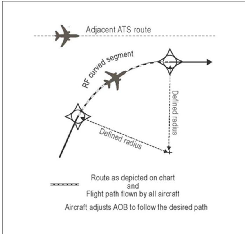
Figure 5-2 (cont.d). Fixed radius transition (FRT) and radius arc to a fix (RF) turn (see 5.4.1.1.4)
