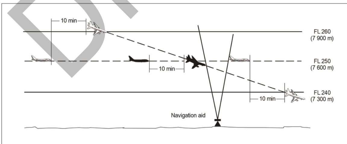
Figure 5-20B. Ten-minute separation between aircraft descending and on crossing tracks
