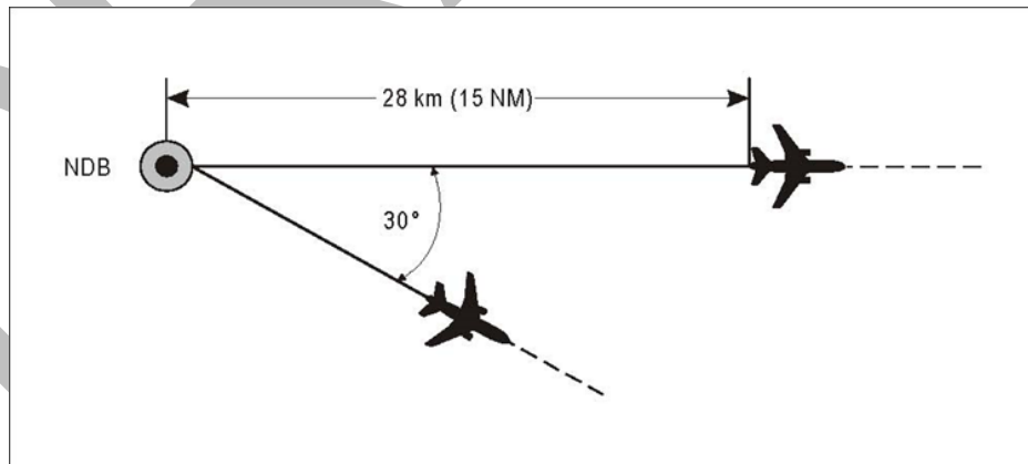
Figure 5-5. Separation using the same NDB (see 5.4.1.2.1.2 b))
