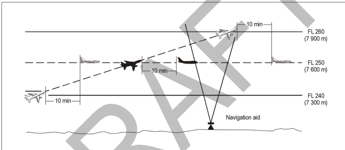
Figure 5-20A. Ten-minute separation between aircraft climbing and on crossing tracks
