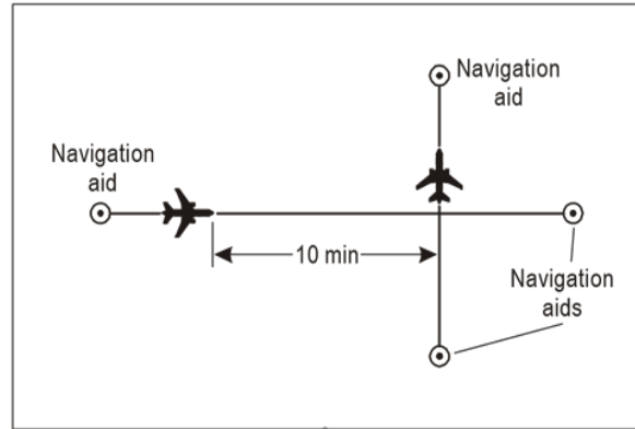
Figure 5-15. Ten-minute separation between aircraft on crossing tracks and same level
