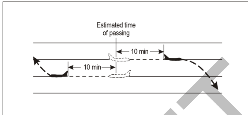
Figure 5-21. Ten-minute separation between aircraft on reciprocal tracks
