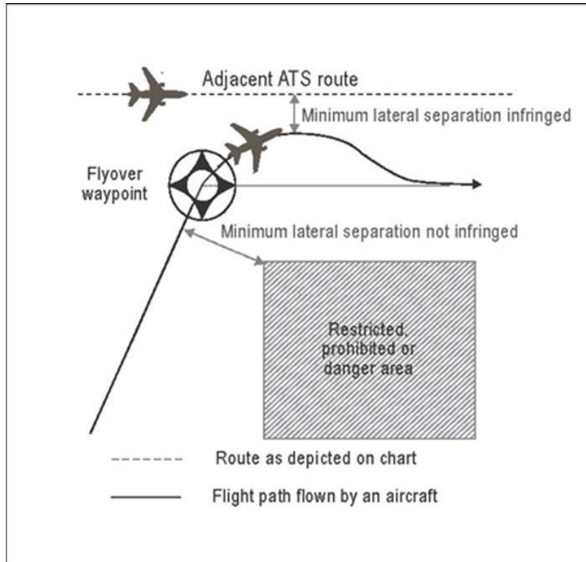
Figure 5-1 (cont.d). Turn over flyover waypoint and turn at fly-by waypoint (see 5.4.1.1.4)
