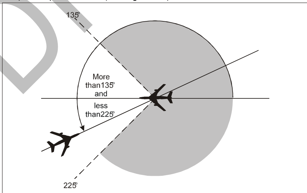
Figure 5-8. Aircraft on reciprocal tracks
