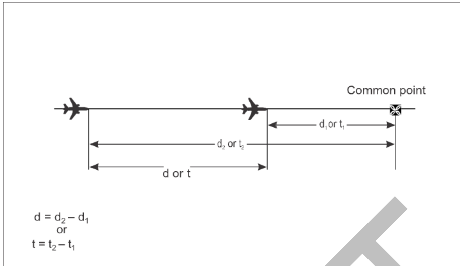
Figure 5-30. Calculation of longitudinal distance/time between aircraft — identical track, same direction
