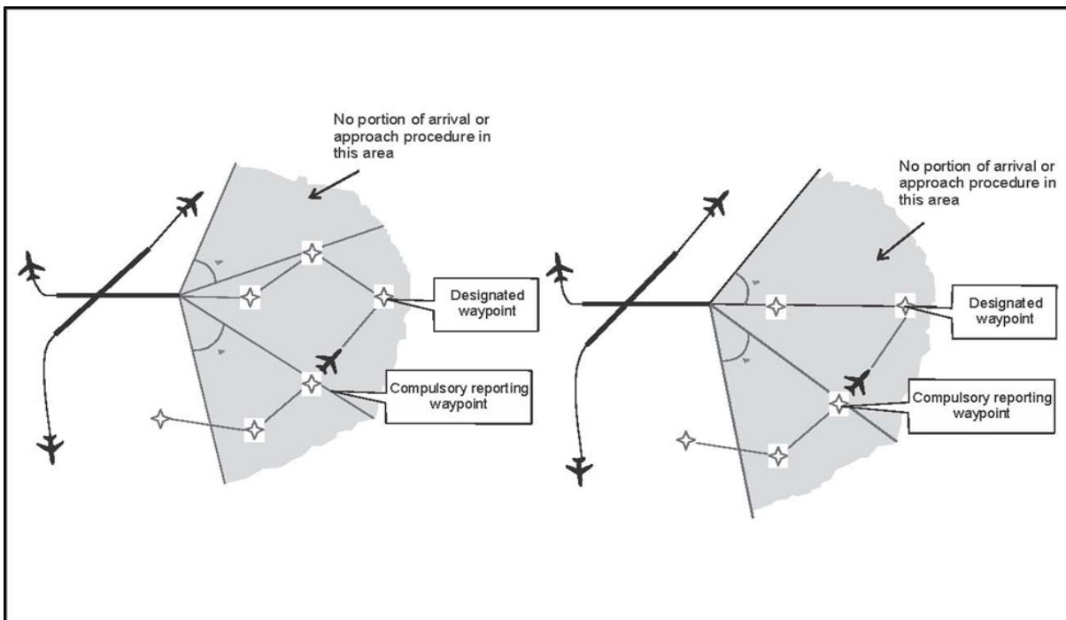
Figure 5-41. Examples of arrival protection area
