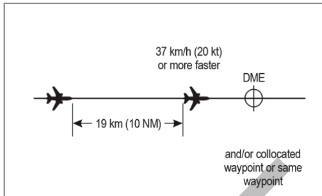
Figure 5-23. 19 km (10 NM) DME and/or GNSS-based separation between aircraft on same track and same level
