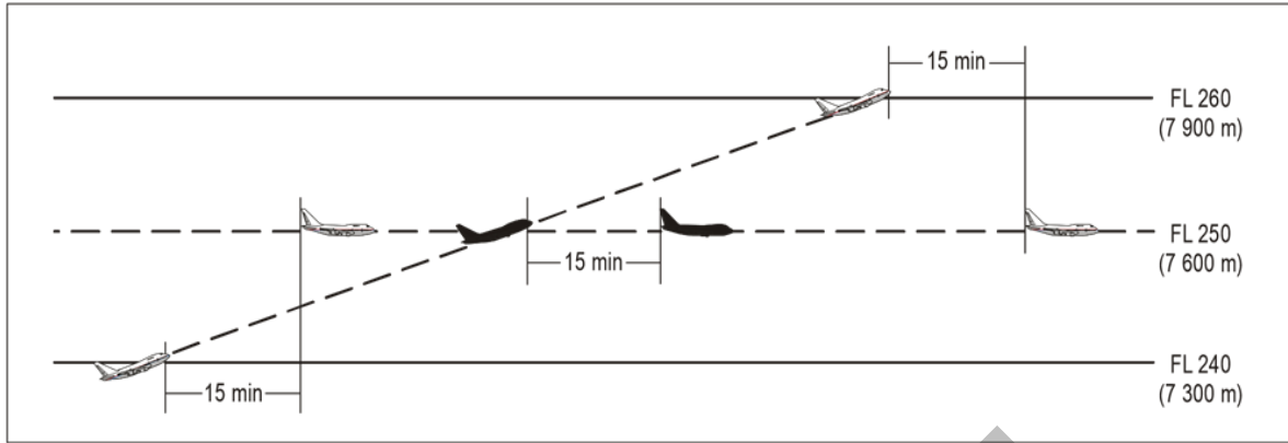
Figure 5-16A. Fifteen-minute separation between aircraft climbing and on same track
