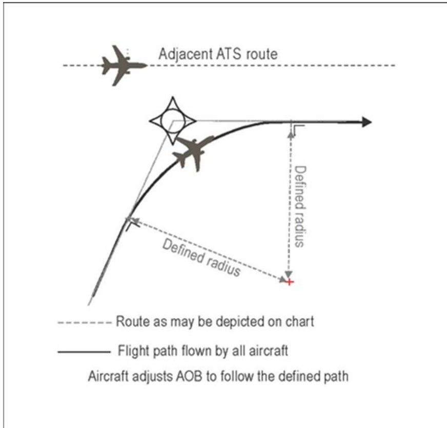
Figure 5-2. Fixed radius transition (FRT) and radius arc to a fix (RF) turn (see 5.4.1.1.4)
