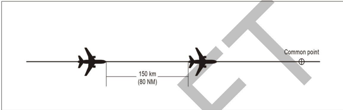
Figure 5-26. 150 km (80 NM) RNAV-based separation between aircraft at the same level
