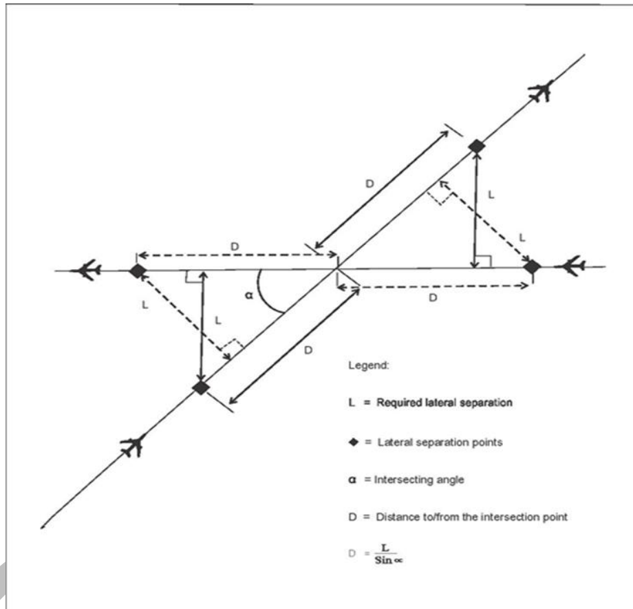
Figure 5-6. Lateral separation points (see 5.4.1.2.1.7)
