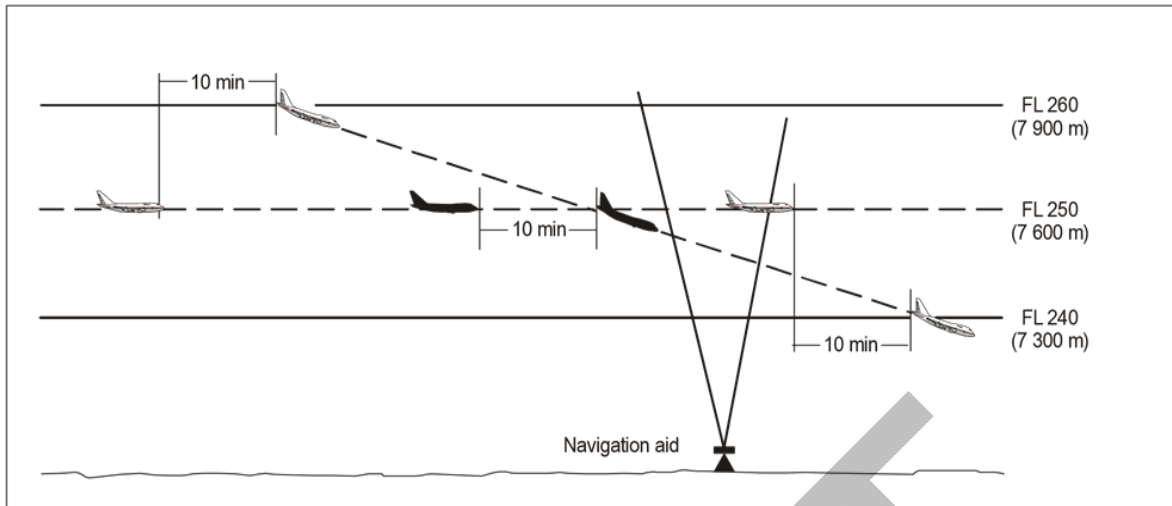
Figure 5-17B. Ten-minute separation between aircraft descending and on same track
