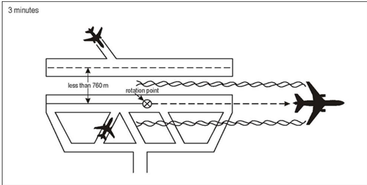
Figure 5-44. Three-minute wake turbulence separation for following aircraft (see 5.8.3.2)
