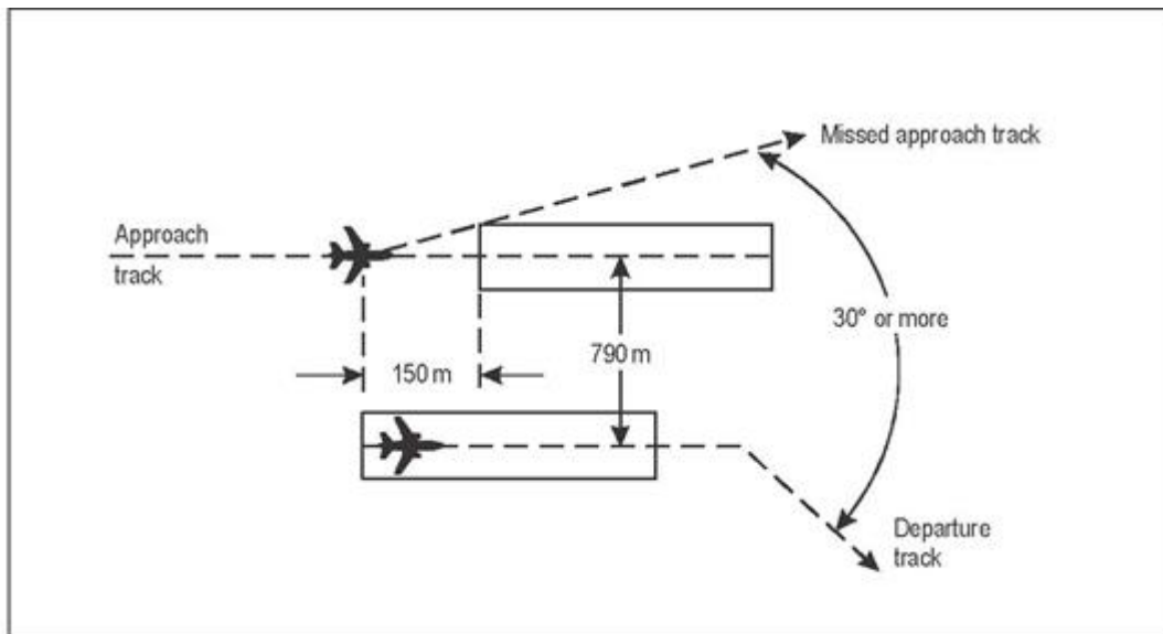
Figure 6-9. Segregated parallel operations where runways are staggered away from the arriving aircraft
