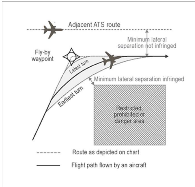
Figure 5-1. Turn over flyover waypoint and turn at fly-by waypoint (see 5.4.1.1.4)
