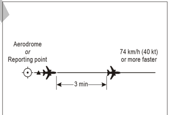
Figure 5-13. Three-minute separation between aircraft on same track and same level
