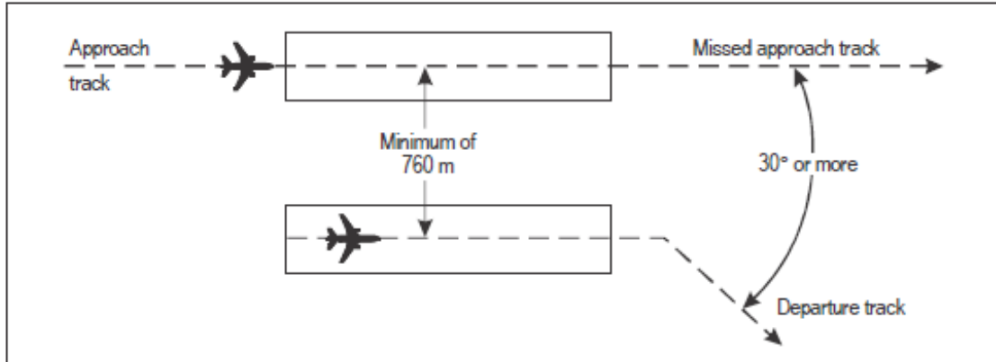
Figure 6-7. Segregated parallel operations
