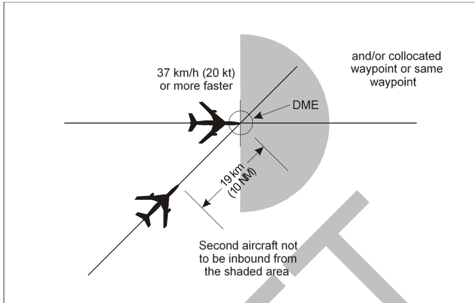
Figure 5-24B. 19 km (10 NM) DME and/or GNSS-based separation between aircraft on crossing tracks and same level
