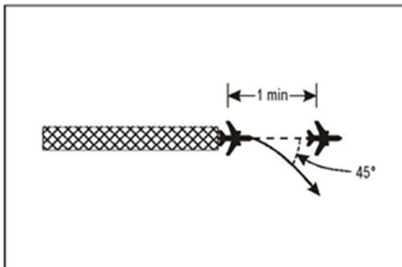
Figure 5-37. One-minute separation between departing aircraft following tracks diverging by at least 45 degrees (see 5.6.1)
