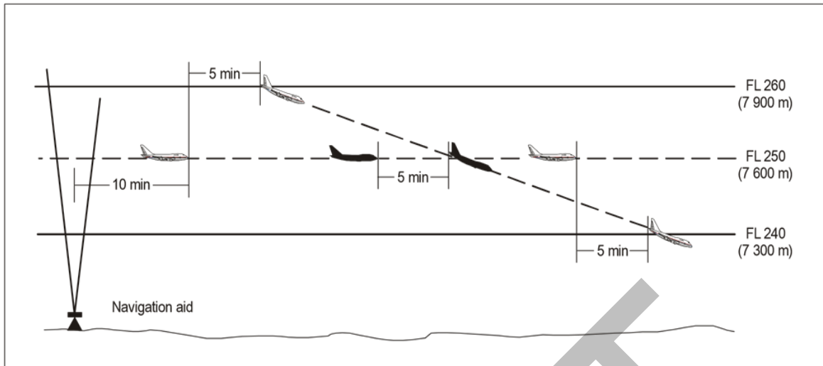
Figure 5-18B. Five-minute separation between aircraft descending and on same track
