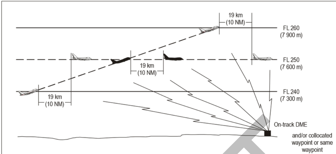
Figure 5-25A. 19 km (10 NM) DME and/or GNSS-based separation between aircraft climbing and on same track
